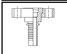
BRIDA POCLAIN MACHO POCLAIN FLANGE MALE
