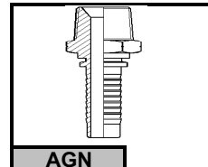
MACHO NPTF NPTF MALE
